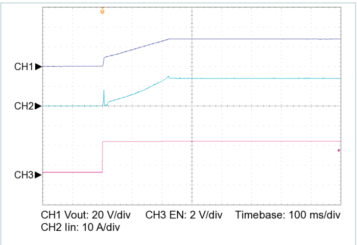
Figure 17 — Startup from EN, V_{IN} = 24\text{ V} , C_{OUT\_EXT} = 10000\ \mu\text{F} , R_{LOAD} = 2.450\ \Omega
