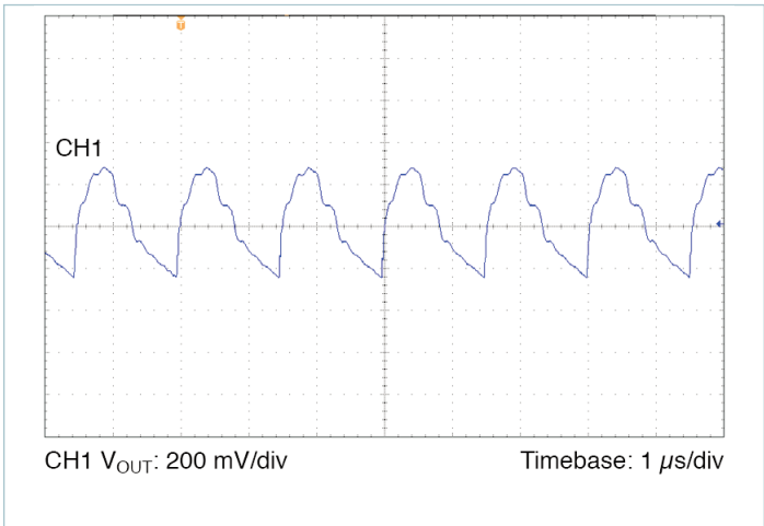
Figure 19 — Output voltage ripple, V_{IN} = 24\text{ V} , V_{OUT} = 28.0\text{ V} , C_{OUT\_EXT} = 1000\ \mu\text{F} , R_{LOAD} = 2.450\ \Omega
