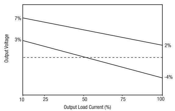
CRE1S0505MEC
