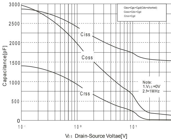
Fig.5 Capacitance Characteristics
