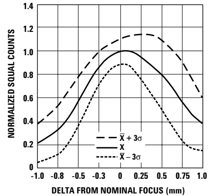
Figure 37. Typical SQUAL vs. Height, Z. (white paper)
