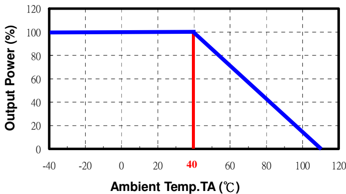
BWC60 Series Power Derating Curve without Heatsink (4)
