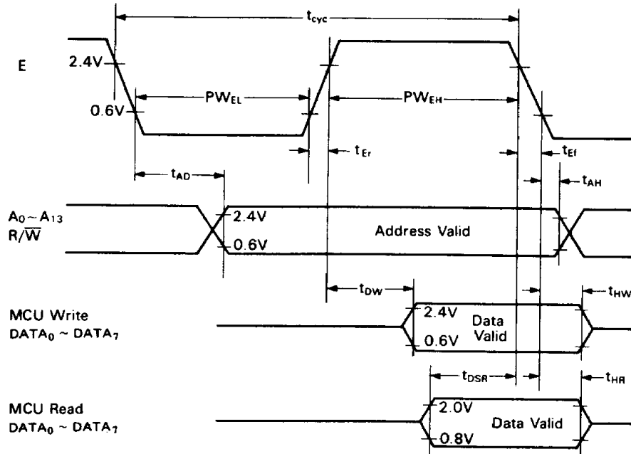
Figure 1 Bus Timing
