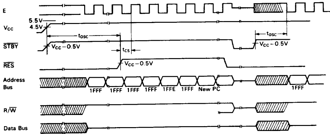
Figure5 Reset Timing
