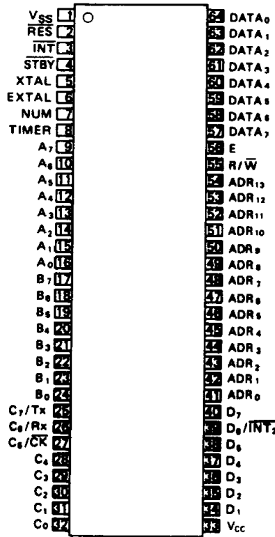
(Top View)
