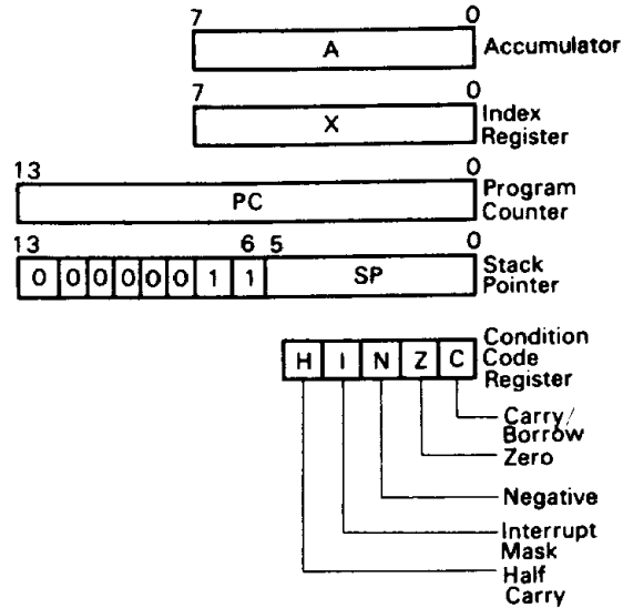
Figure 11 Programming Model
