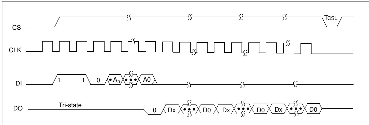
FIGURE 2-2: READ TIMING
