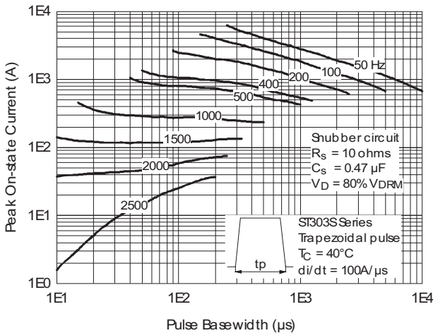
Fig. 13 - Frequency Characteristics
