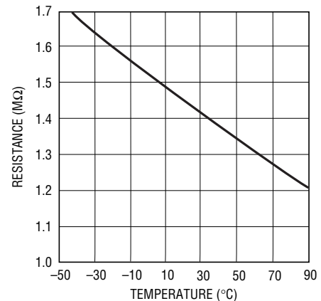
EN_CHRG Pin Pulldown Resistance vs Temperature
