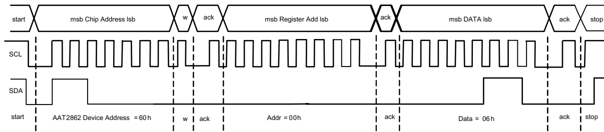
Figure 1: Typical I²C Timing Diagram.
