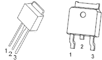
TO-251-3L/TO-252-2L
