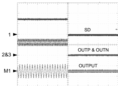
Shutdown
