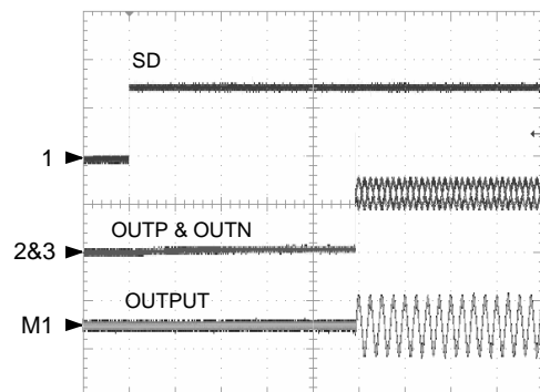
Shutdown Release
