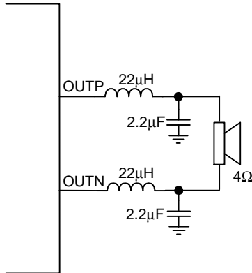
Figure 4. LC output filter for 4Ω speaker Inductor : TOKO 11RHBP A7503AY-220M
