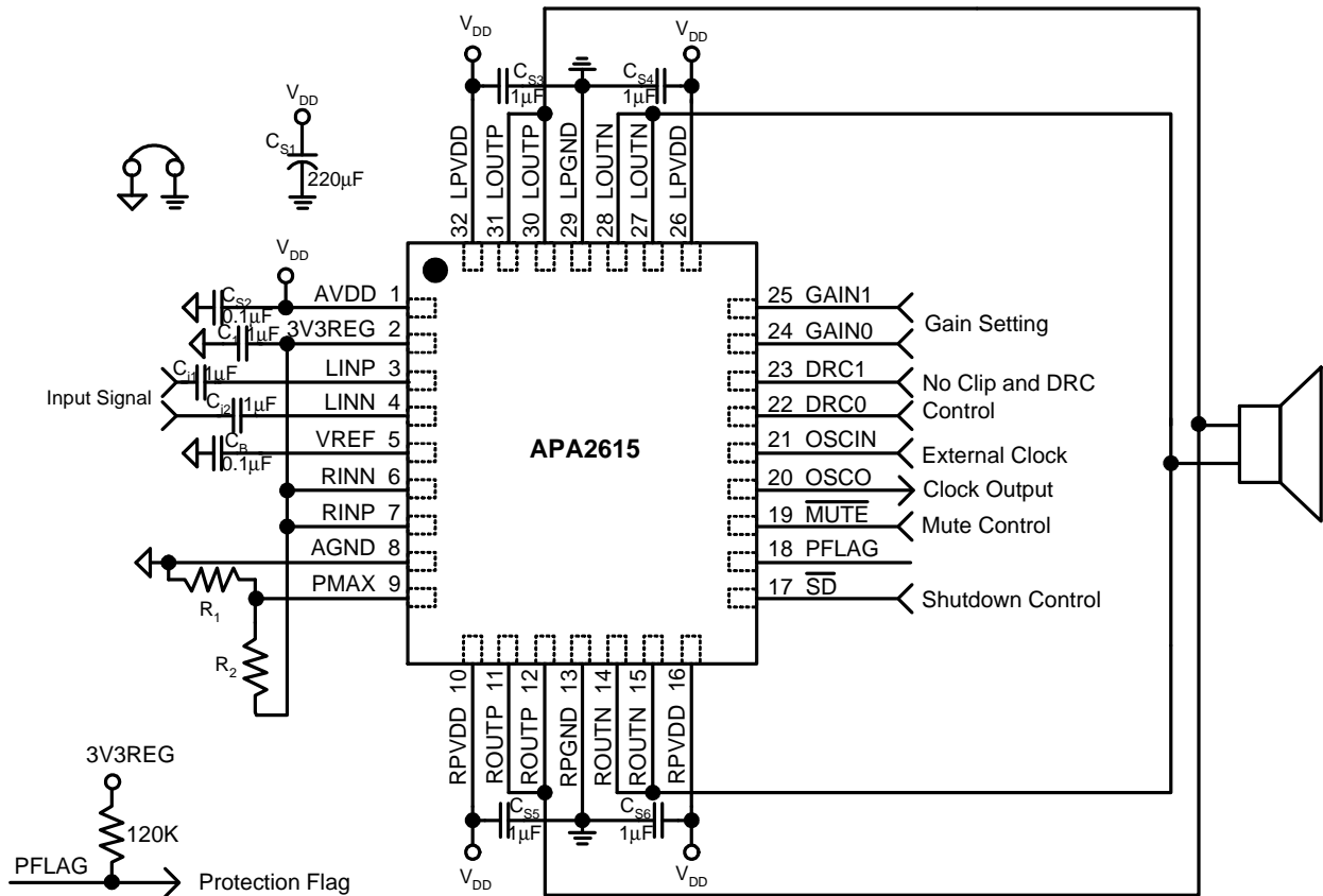
Monaural Operation
