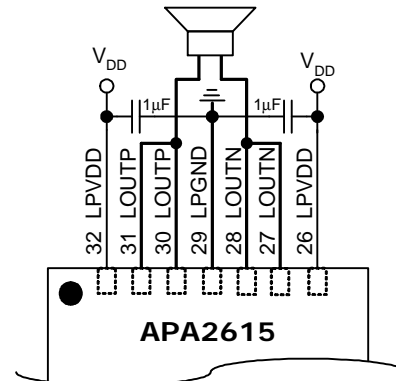
Figure 5. APA2615 Output Topology
