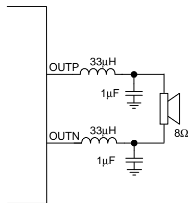
Figure 3. LC output filter for 8 \Omega speaker Inductor :TOKO 11RHBP A7503AY-330M
