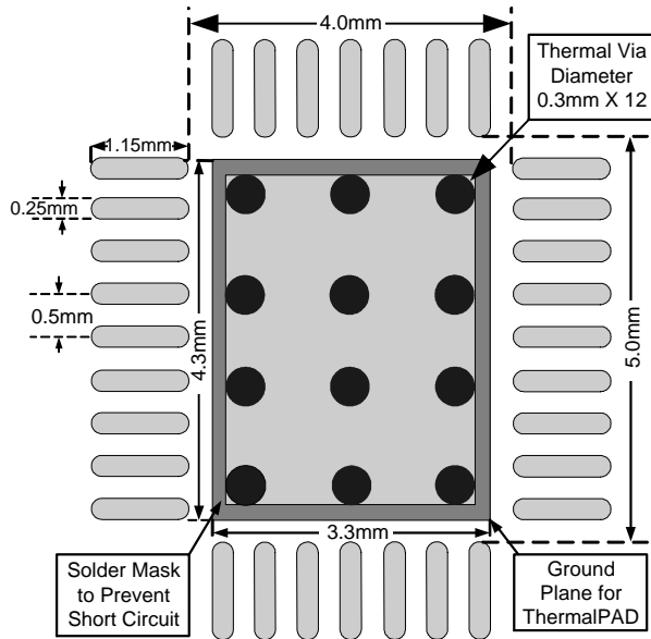
Figure 6. QFN5.2x6.2-32 Land Pattern Recommendation
