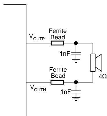
Figure 2. Ferrite bead output filter
