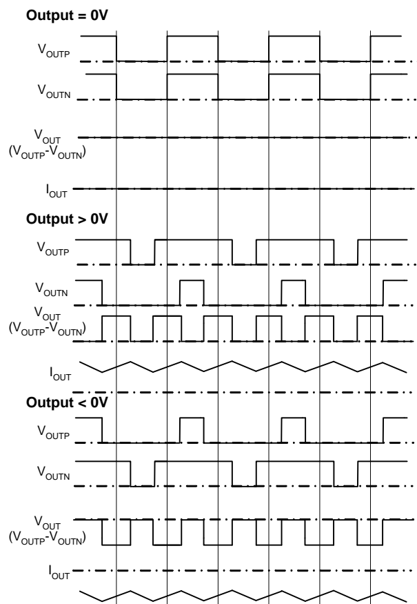
Figure 1. The APA2615 Output Waveform (Voltage & Current)
