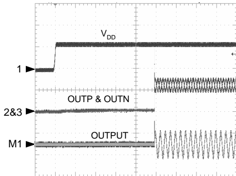
Power On
