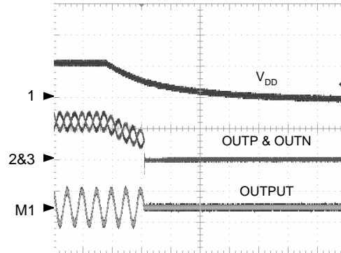
Power Off
