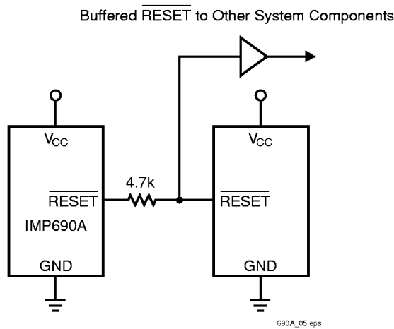
Figure 3. Interfacing with bi-directional microprocessor reset inputs
