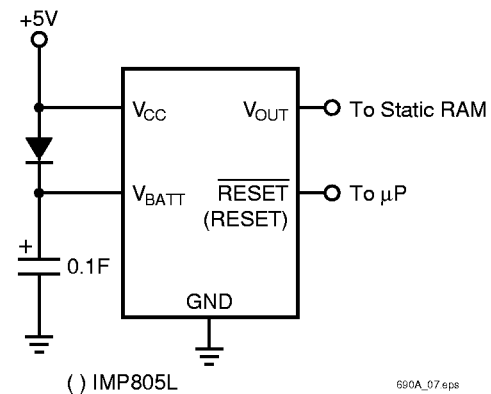
Figure 5. Capacitor as a backup power source
