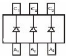
BAT54T
