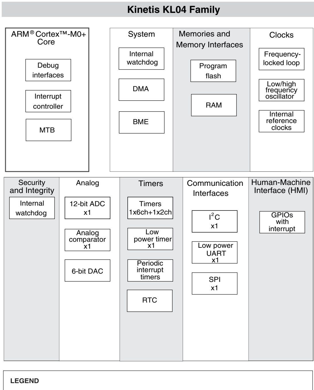
Figure 2. KL04 Family Block Diagram
