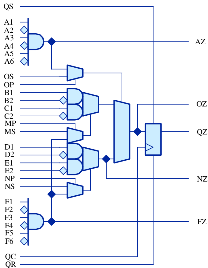
Figure 4: Logic Cell
