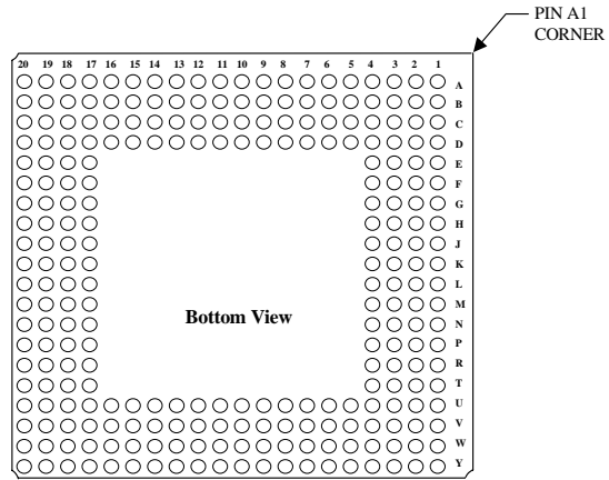
Figure 9: 256-pin PBGA
