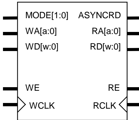
Figure 5: RAM Module
