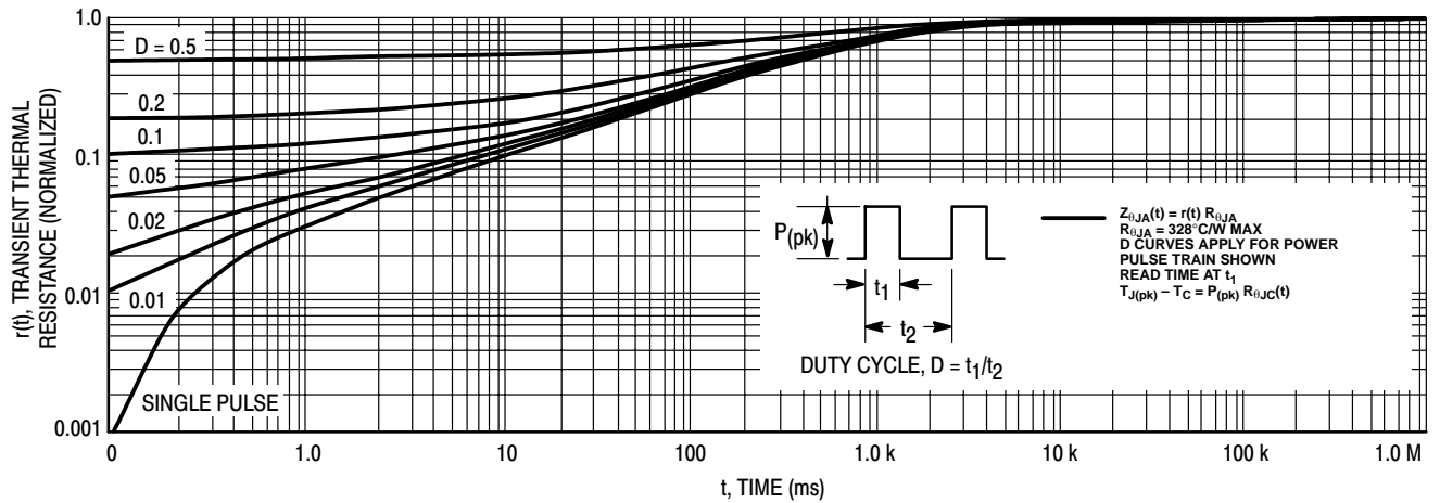
Figure 25. Thermal Response
