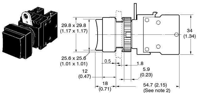
Square/Extended Type A22-C, A22L-C
