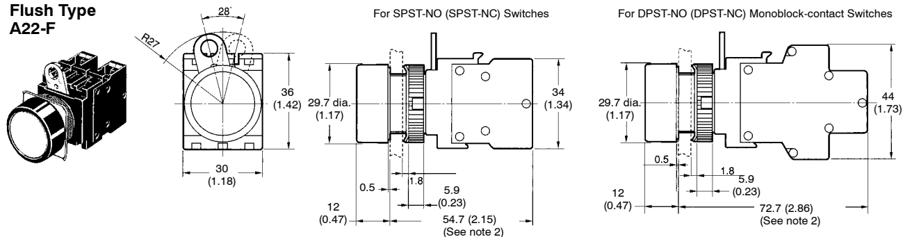
Half-guard Type A22-H, A22L-H
