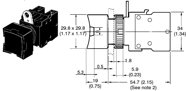
Square Flush Type A22-D, A22L-D
