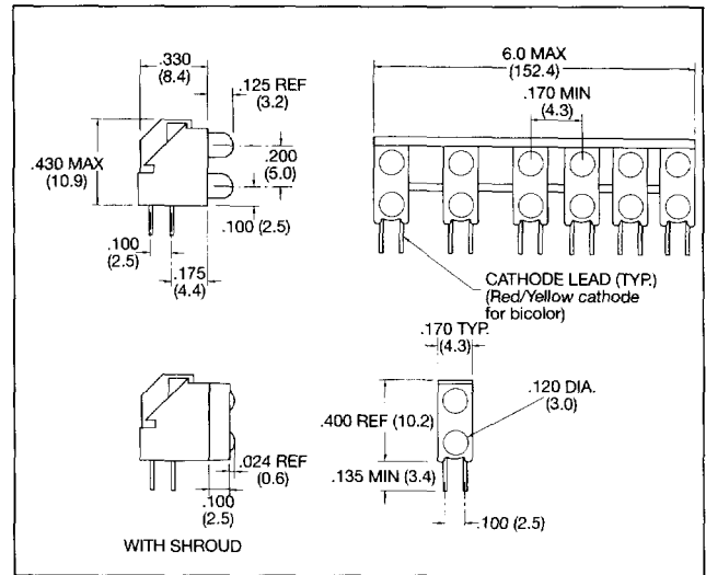
All Dimensions are in inches (mm) Standard Polarity shown in drawing: Cathode right
