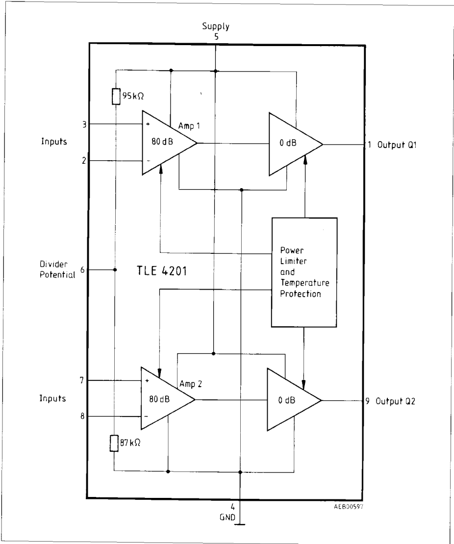
Figure 1 Block Diagram
