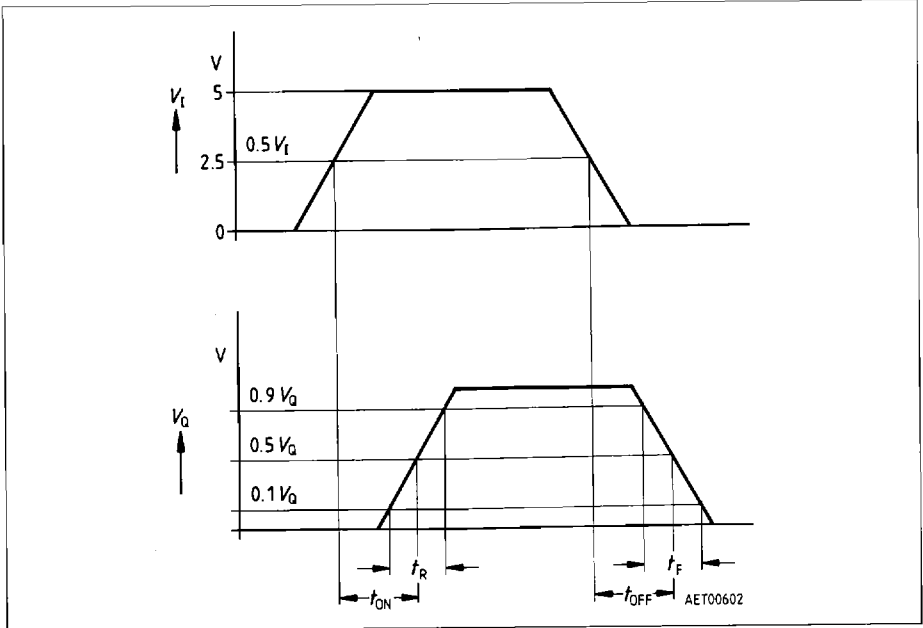
Figure 6 Pulse Diagram
