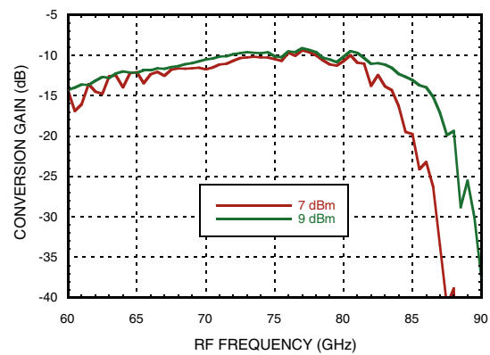
Conversion Gain vs. LO Power LO= 4 GHz, LSB
