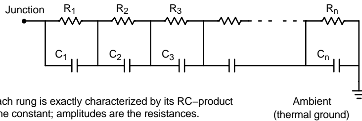
Figure 16. Non-Grounded Capacitor Thermal Ladder ("Foster" Ladder)
