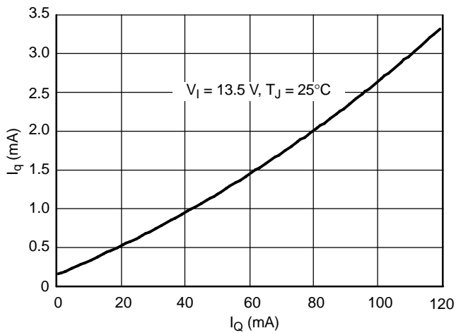
Figure 7. Current Consumption I_q vs. Output Current I_Q
