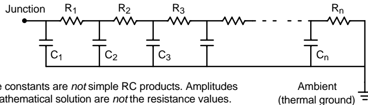
Figure 15. Grounded Capacitor Thermal Network ("Cauer" Ladder)
