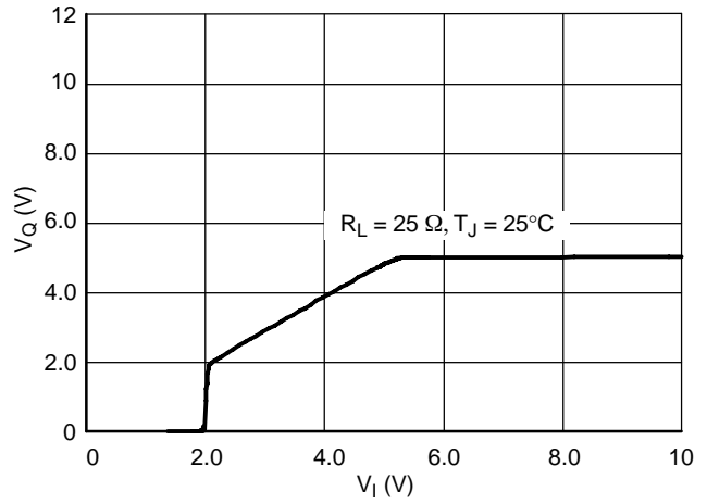
Figure 4. Output Voltage V_Q vs. Input Voltage V_I
