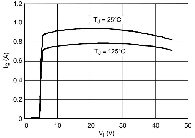
Figure 6. Output Current I_Q vs. Input Voltage V_I
