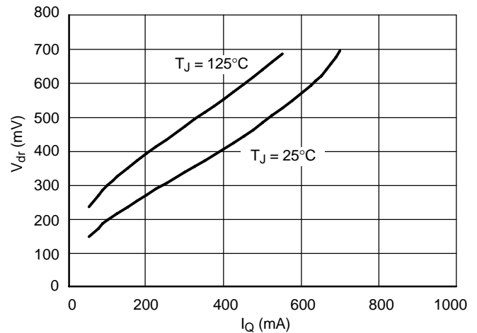
Figure 8. Drop Voltage V_{dr} vs. Output Current I_Q
