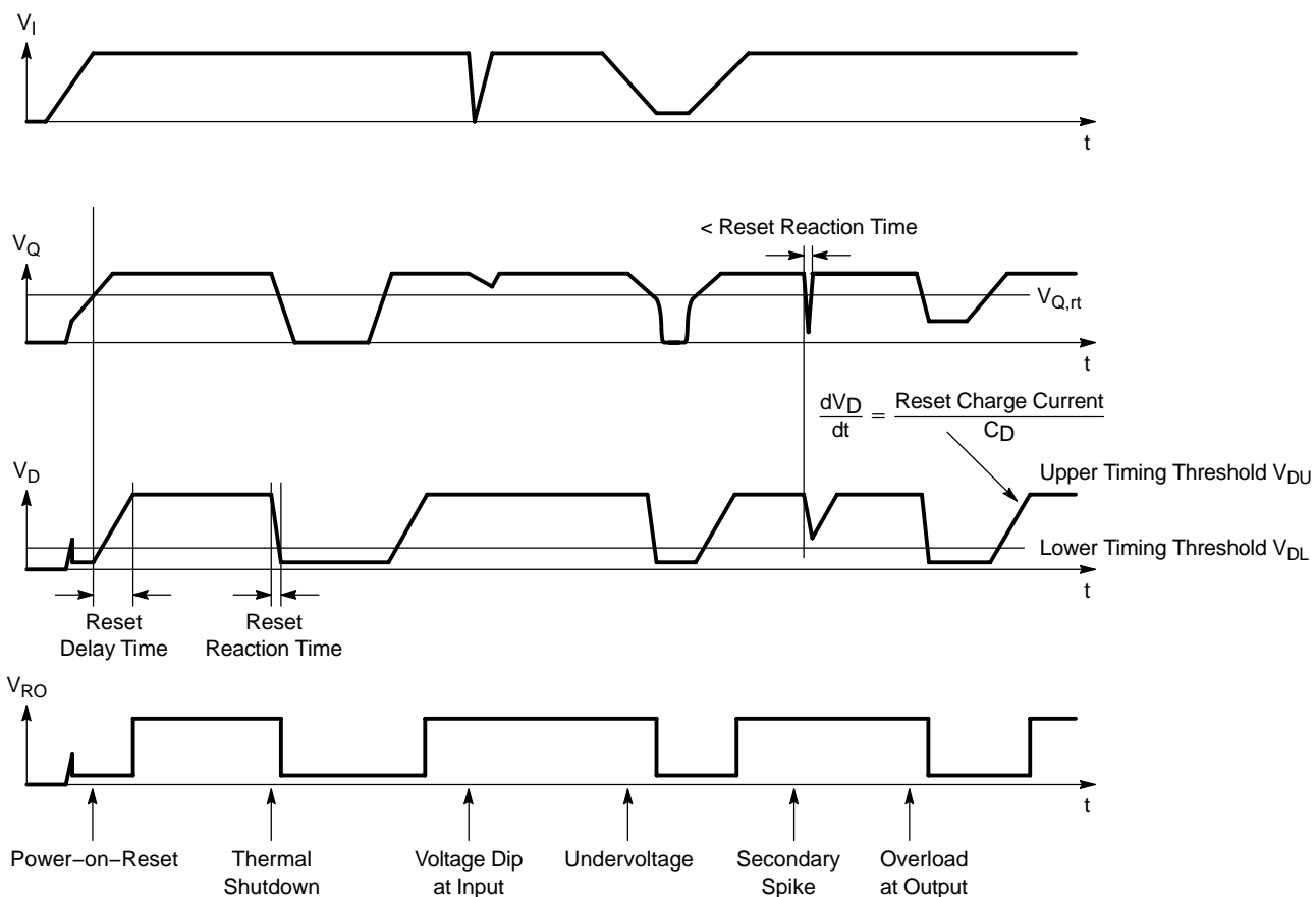
Figure 13. Reset Timing
