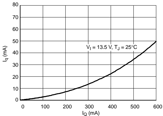
Figure 9. Current Consumption I_q vs. Output Current I_Q
