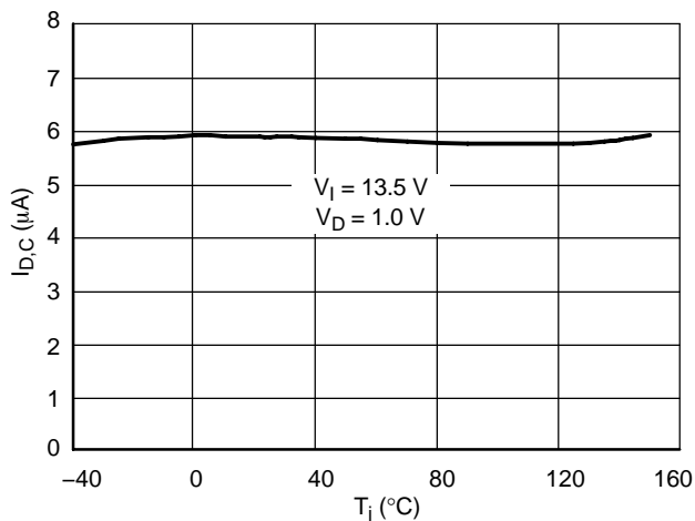
Figure 10. Charge Current I_{D,C} vs. Temperature T_J
