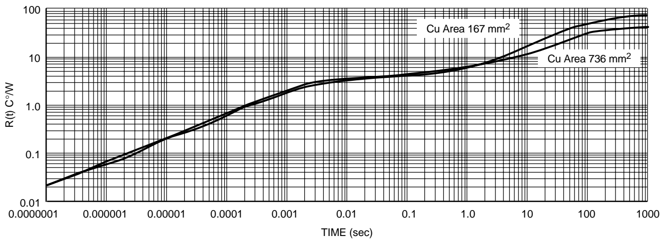
Figure 20. Single-Pulse Heating Curves, \text{D}^2\text{PAK} 5-Lead
