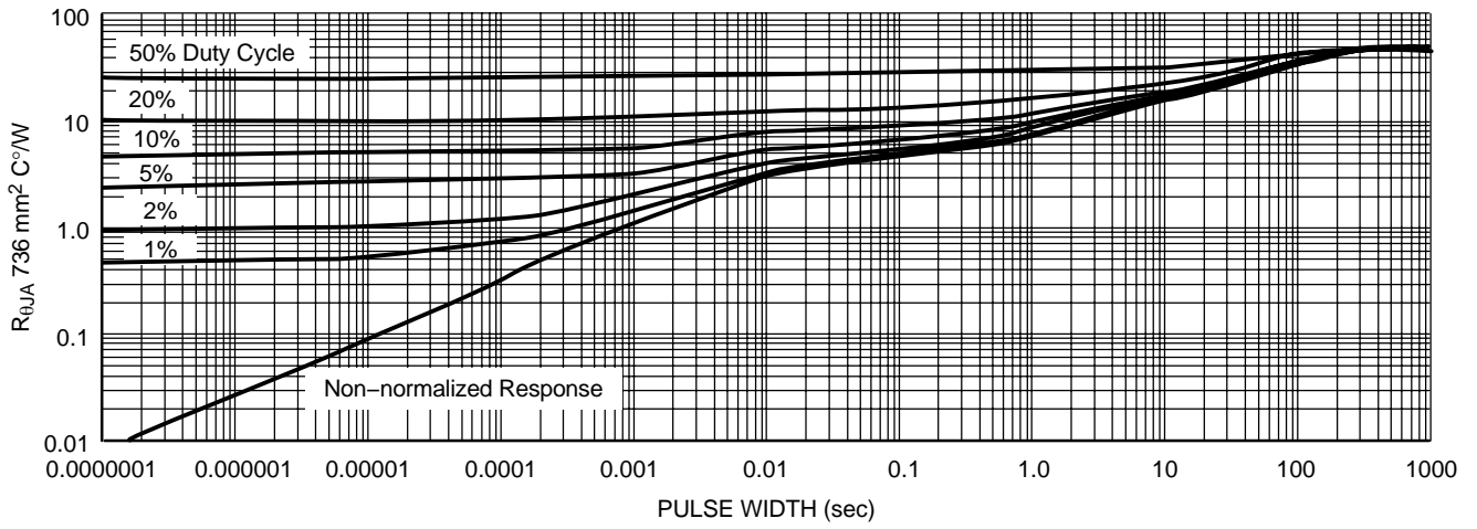
Figure 21. Duty Cycle for 1" Spreader Boards, DPAK 5-Lead
