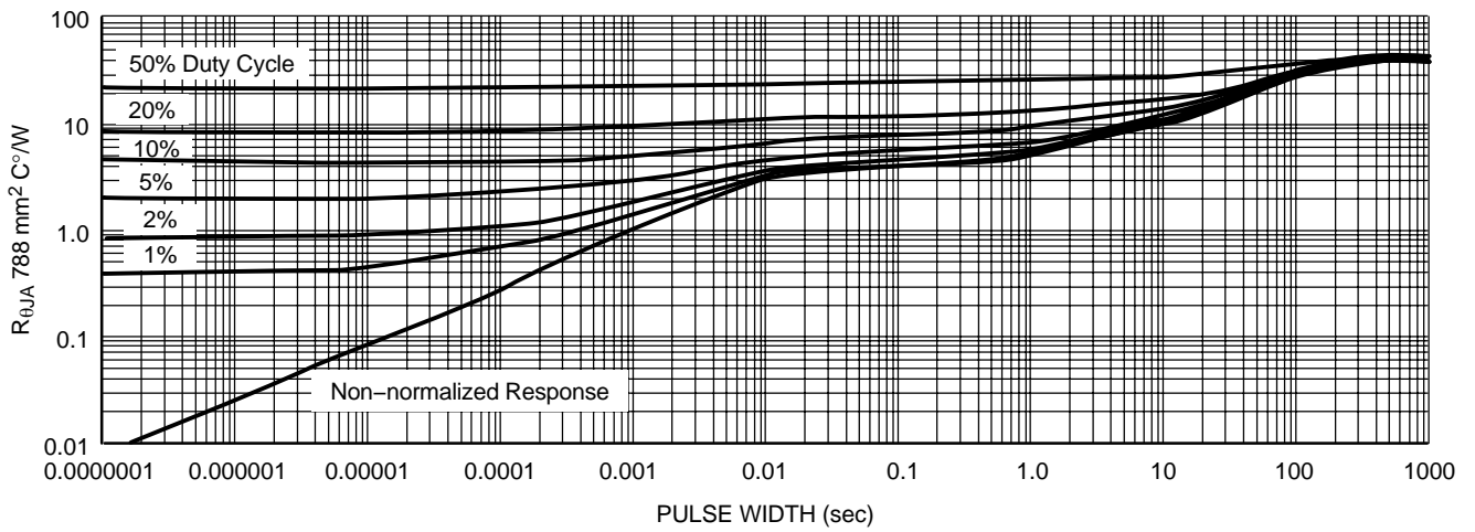
Figure 22. Duty Cycle for 1" Spreader Boards, D 2 PAK 5-Lead
