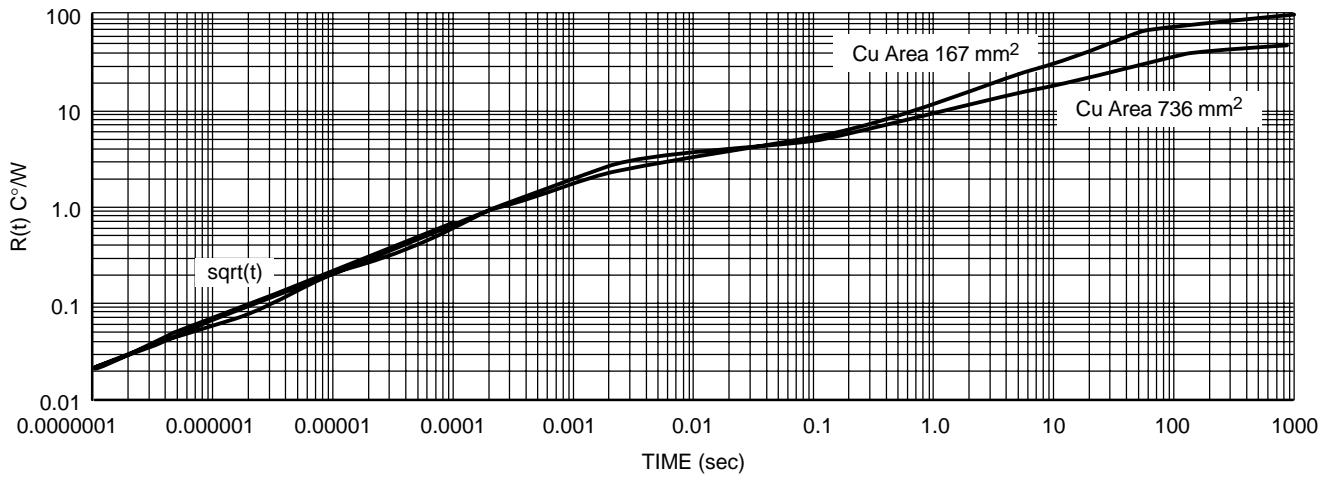
Figure 19. Single-Pulse Heating Curves, DPAK 5-Lead
