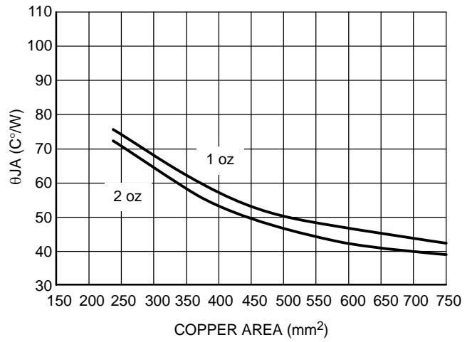
Figure 18. \theta_{JA} vs. Copper Spreader Area, \text{D}^2\text{PAK} 5-Lead
