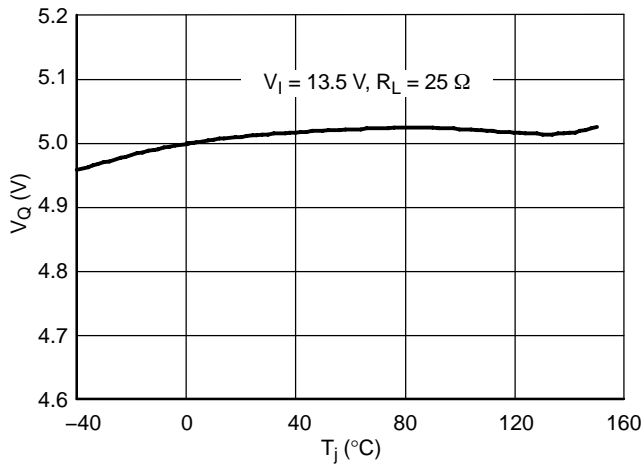
Figure 3. Output Voltage V_Q vs. Temperature T_J
