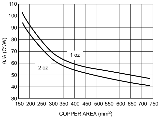
Figure 17. \theta_{JA} vs. Copper Spreader Area, DPAK 5-Lead
