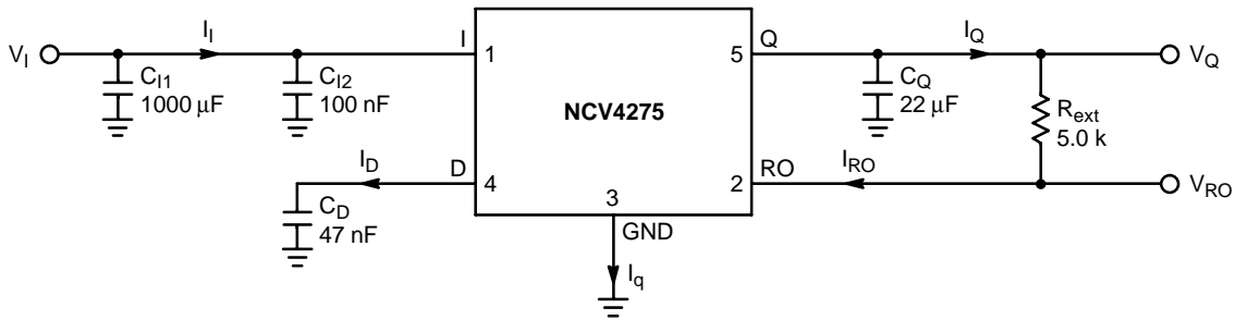
Figure 12. Test Circuit
