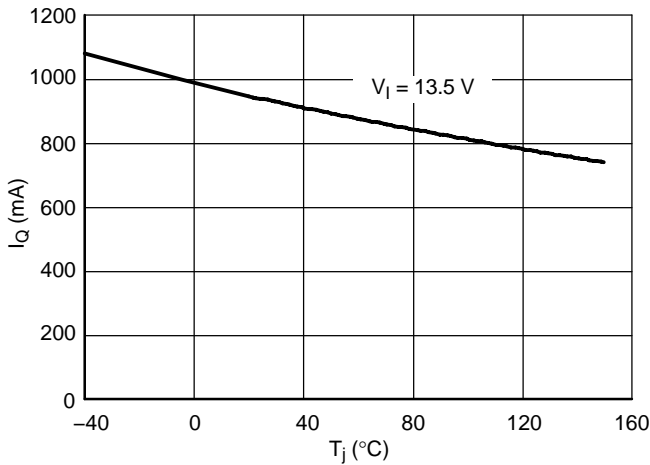
Figure 5. Output Current I_Q vs. Temperature T_J
