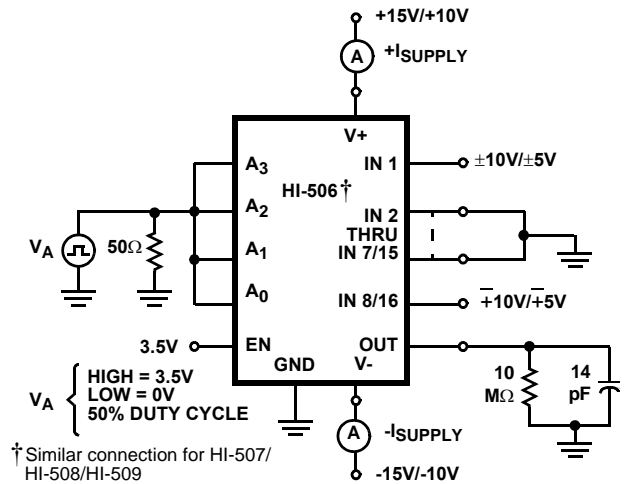
FIGURE 4B. TEST CIRCUIT
