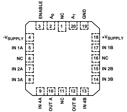
HI-509 (PLCC) TOP VIEW
