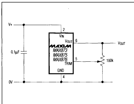
Figure 2. Output-Voltage Trim Circuit
