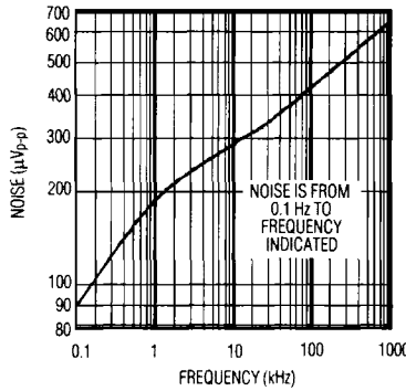
MAX875 WIDEBAND OUTPUT NOISE vs. BANDWIDTH
