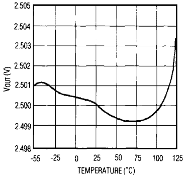
MAX873 OUTPUT VOLTAGE vs. TEMPERATURE
