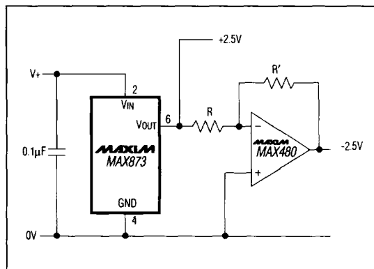
Figure 3. +2.5V and -2.5V Outputs
