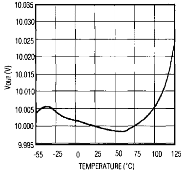
MAX876 OUTPUT VOLTAGE vs. TEMPERATURE
