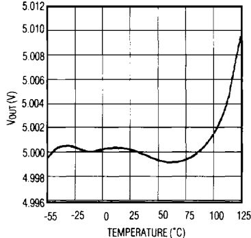
MAX875 OUTPUT VOLTAGE vs. TEMPERATURE
