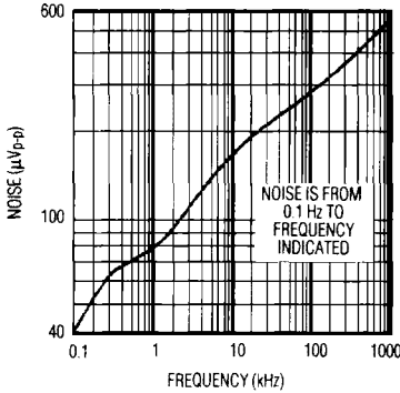
MAX873 WIDEBAND OUTPUT NOISE vs. BANDWIDTH
