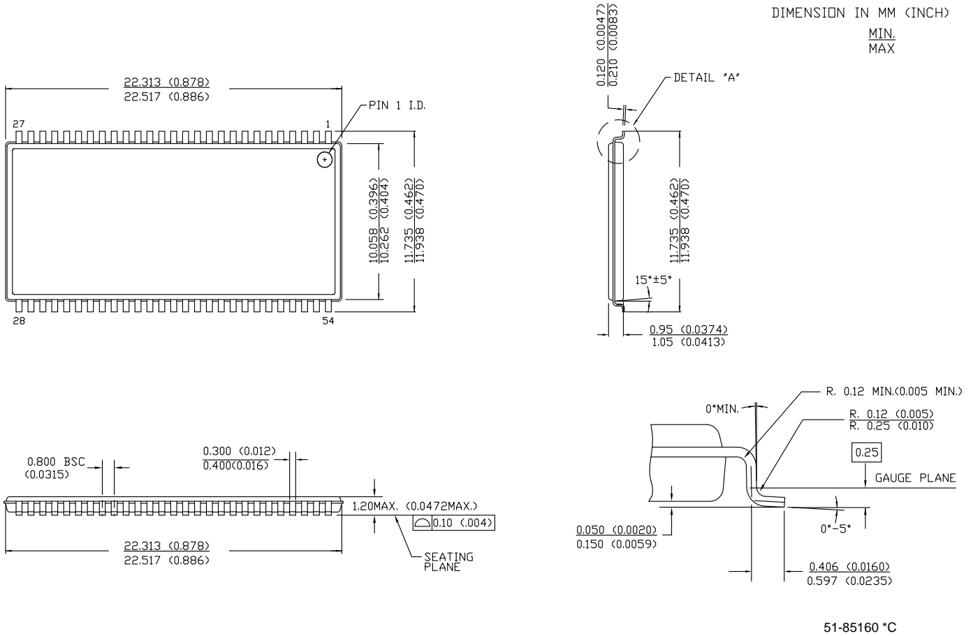
Figure 18. 54-pin TSOP II (22.4 x 11.84 x 1.0 mm), 51-85160
