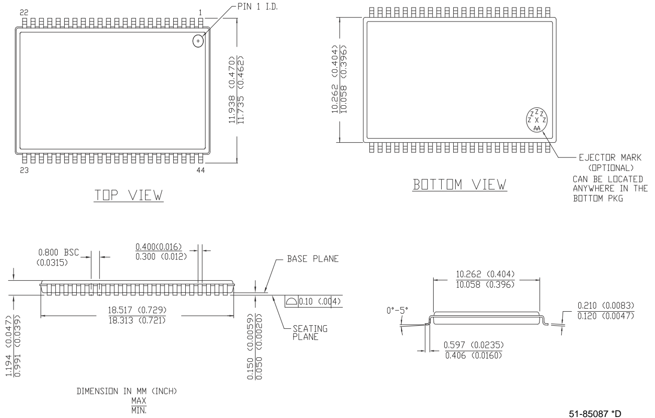
Figure 16. 44-pin TSOP II, 51-85087
