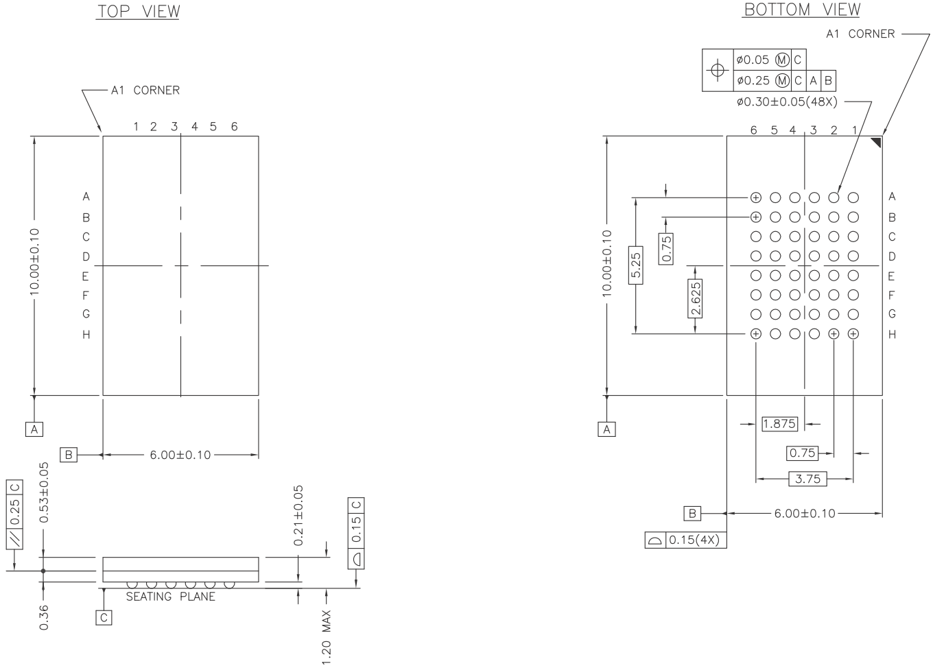
Figure 17. 48-ball FBGA (6 × 10 × 1.2 mm), 51-85128
