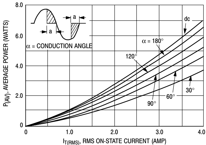
Figure 4. Power Dissipation
