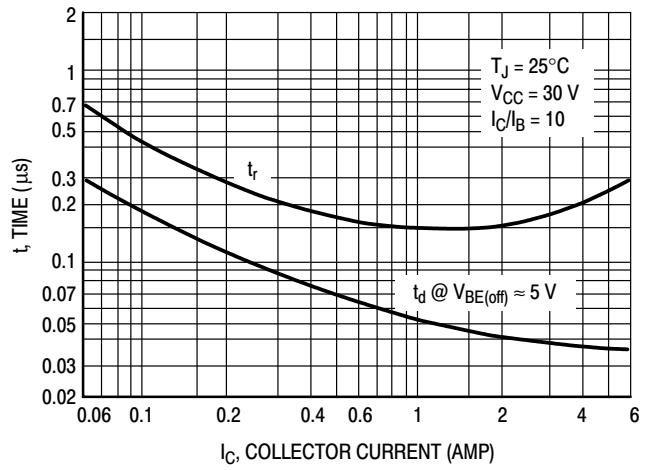
Figure 3. Turn-On Time
