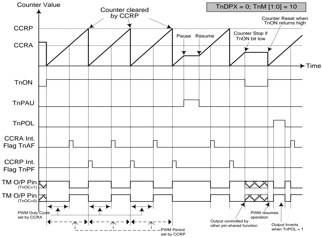
PWM Mode – TnDPX=0
