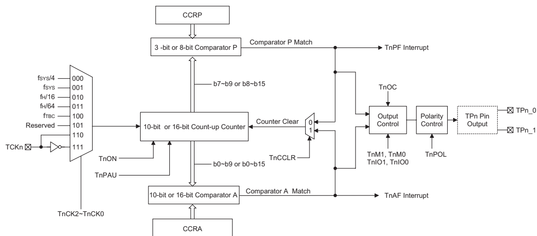
Compact Type TM Block Diagram (n=0, 1, 2, 3, 5)
