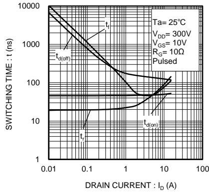
Fig.14 Switching Characteristics
