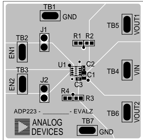
Figure 76. Example 8-Lead LFCSP PCB Layout
