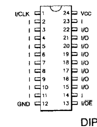
Pin Configuration (Figure 1)
