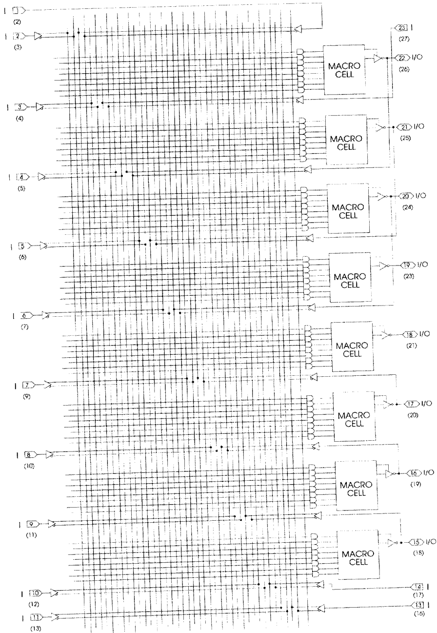
Figure 6. PEEL20V8 Logic Array - Simple Mode (Pin numbers are for DIP and SOIC packages, PLCC pin numbers shown in parentheses.)
