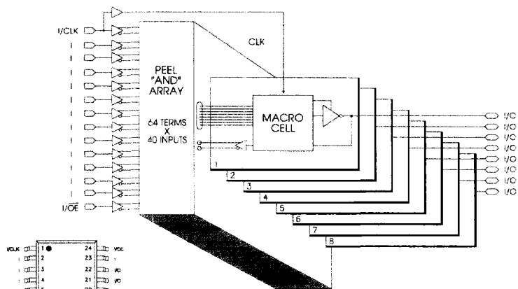
Block Diagram (Figure 2)
