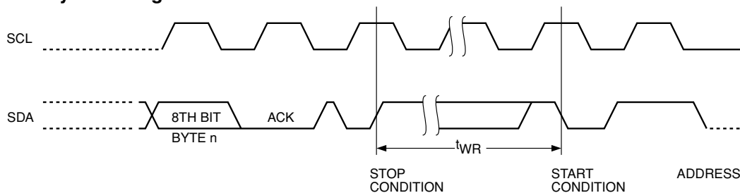
Figure 3. Start/Stop Timing
