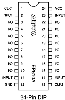
Figure 14. EP610A Package Pin-Out Diagrams
