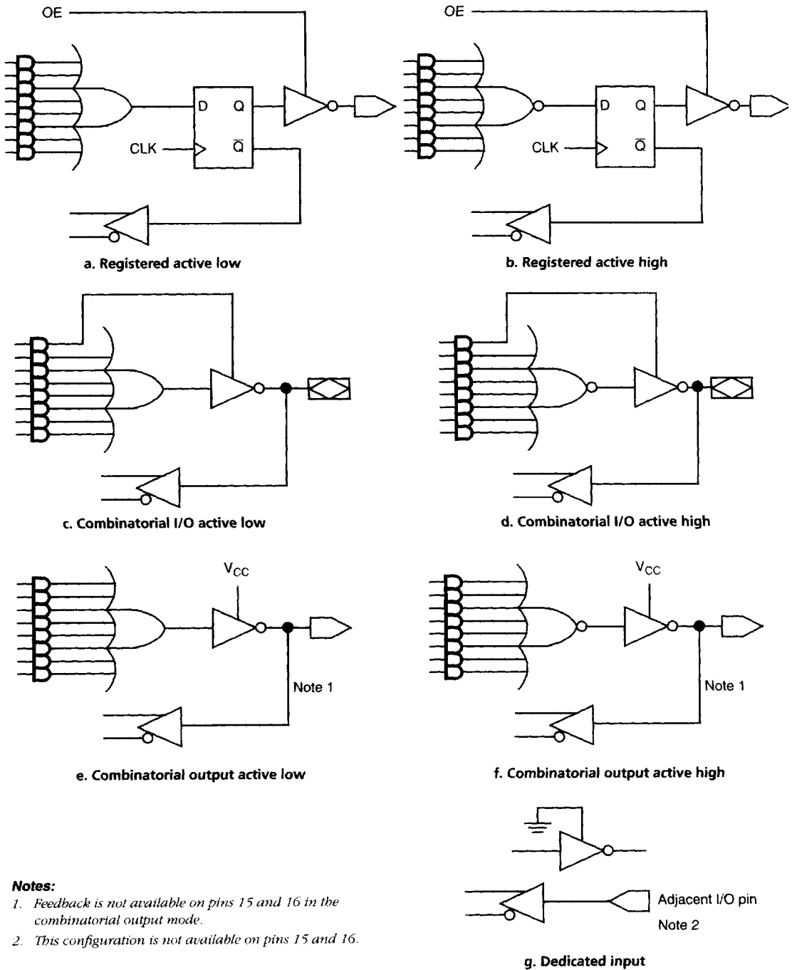
Figure 2. Macrocell Configurations
