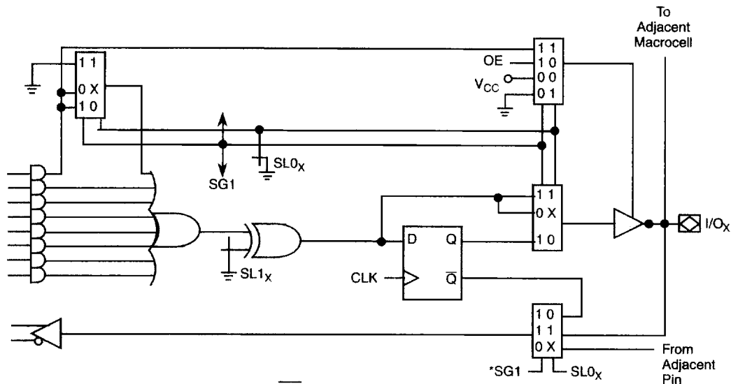
Figure 1. PALCE16V8 Macrocell
