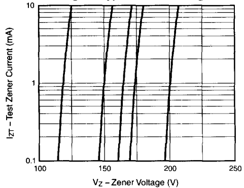
Fig. 6 – Typical Zener Voltage
