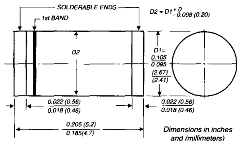
DO-213AB
