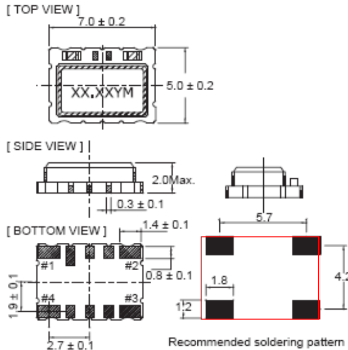
Contact Pads are gold over nickel
