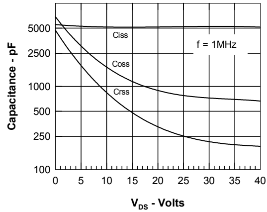
Fig. 8. Capacitance Curves
