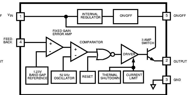
Adjustable Regulator
