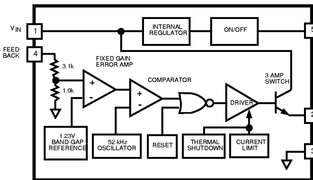
Fixed Regulator
