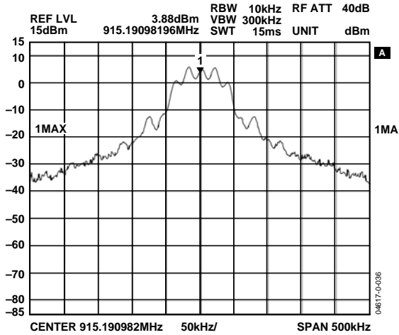
Figure 22. FSK Modulation, Power = 10 dBm, Data Rate = 38.4 kbps, F_{\text{deviation}} = \pm 19.2 \text{ kHz}
