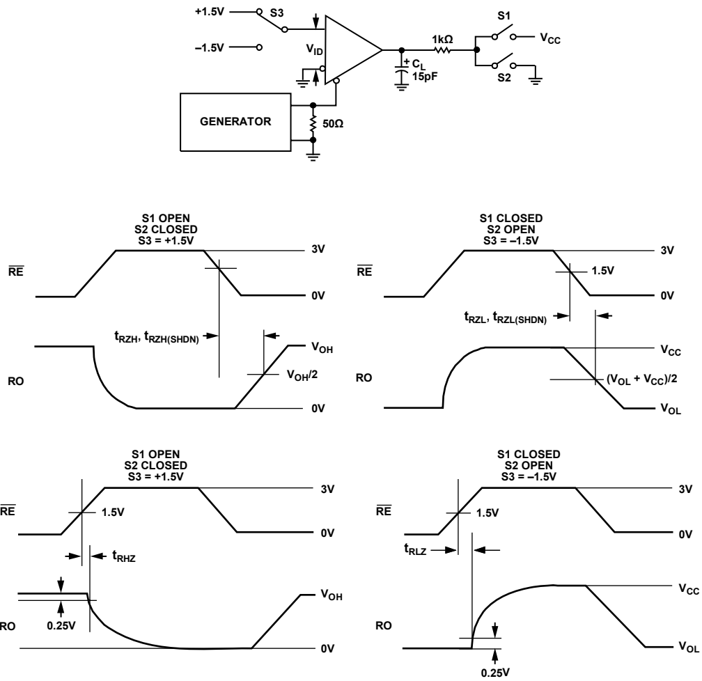
Figure 14. Receiver Enable and Disable Times
