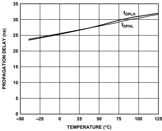
Figure 27. ADM3076E/ADM3077E/ADM3078E Driver Propagation Delay vs. Temperature (16 Mbps)
