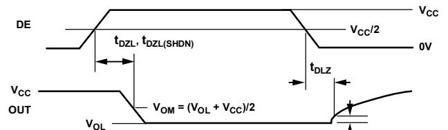
Figure 11. Driver Enable and Disable Times ( t_{DZL} , t_{DLZ} , t_{DZL(SHDN)} )
