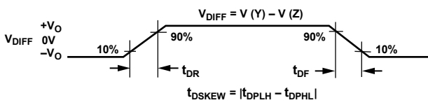
Figure 9. Driver Propagation Delays
