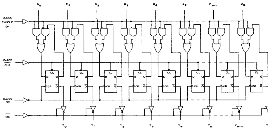
FIGURE 3. Logic diagram.
