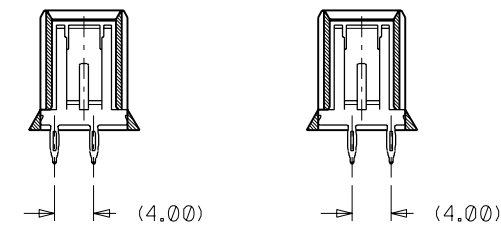
SECTION: Y-Y
