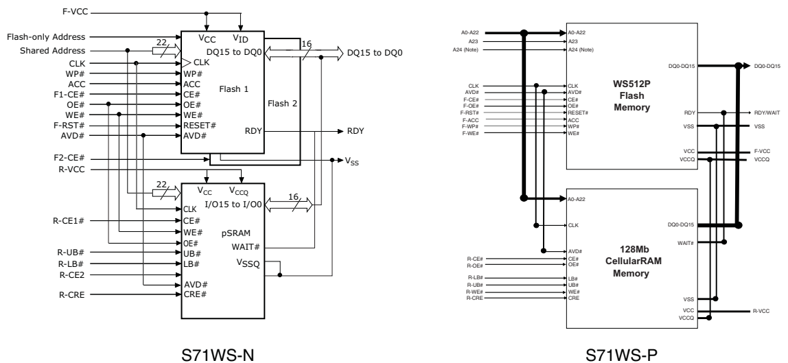
Figure 3.1 Block Diagrams
