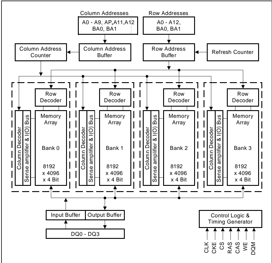
Block Diagram for 128M x 4 SDRAM ( 13 / 12 / 2 addressing)
