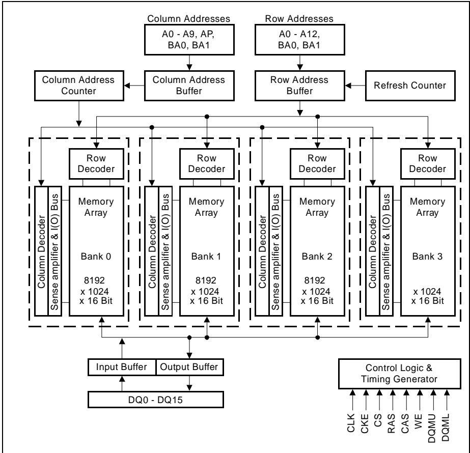
Block Diagram for 32M x 16 SDRAM ( 13 / 10 / 2 addressing)
