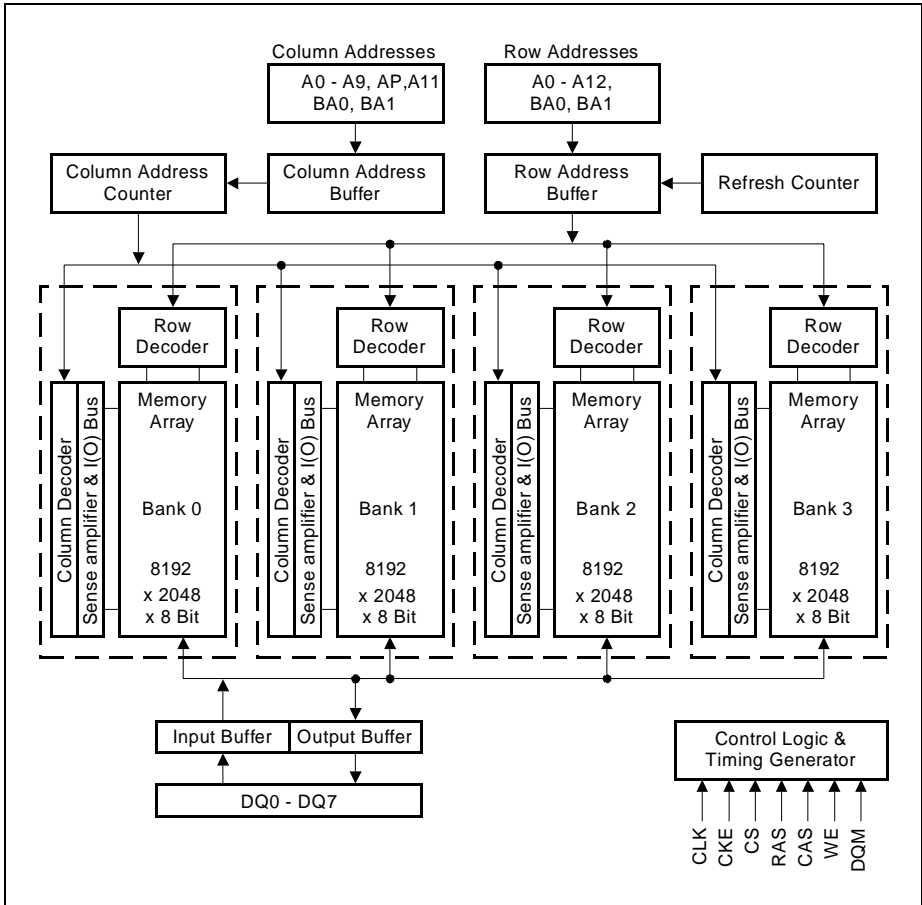
Block Diagram for 64M x 8 SDRAM ( 13 / 11 / 2 addressing)
