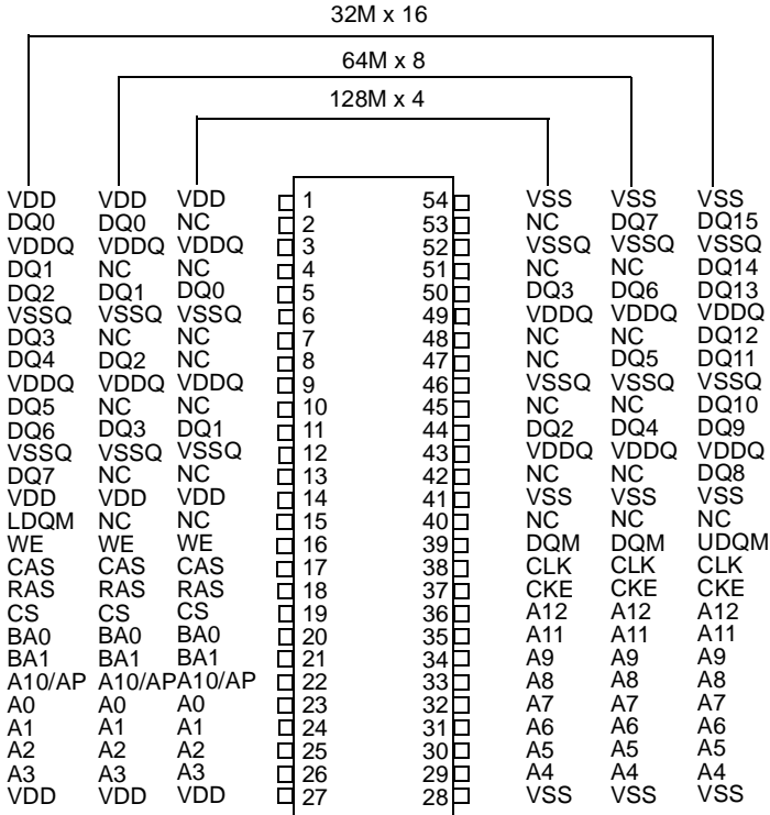
TSOPII-54 (400 mil x 875 mil, 0.8 mm pitch)
