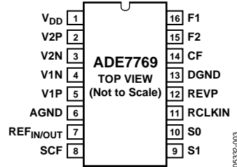
Figure 3. Pin Configuration
