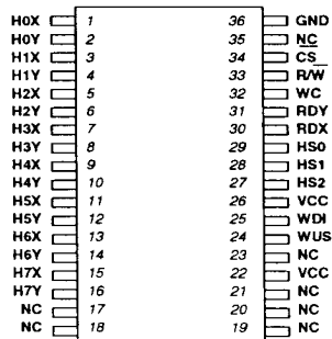
8-Channel 36-lead SOIC
