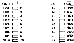
4-Channel 20-lead SOIC, SSOP, VSOP
