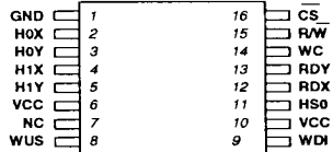
2-Channel 16-lead SOIC
