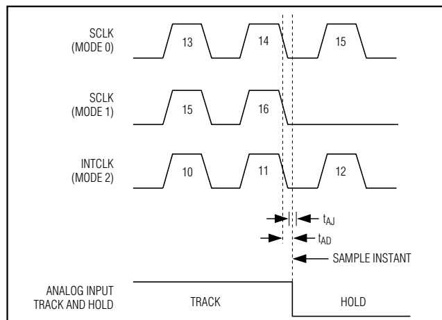
Figure 21. Aperture Diagram
