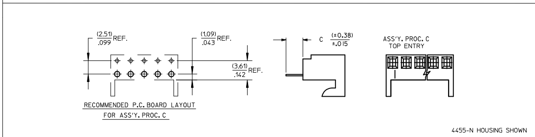
4455-N HOUSING SHOWN
