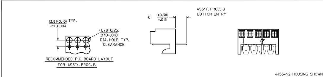
4455-N2 HOUSING SHOWN
