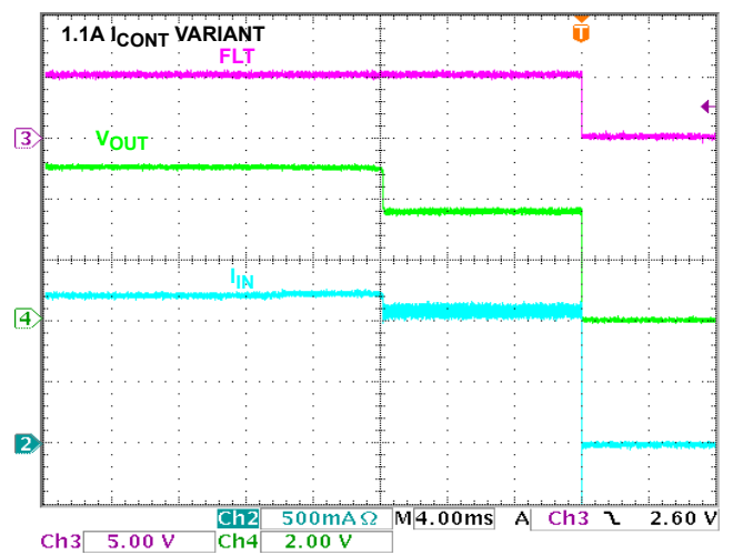
FIGURE 22. I_{LIM} WAVEFORM
