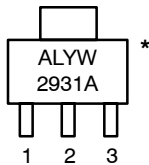
SOT-223 ST SUFFIX CASE 318H
